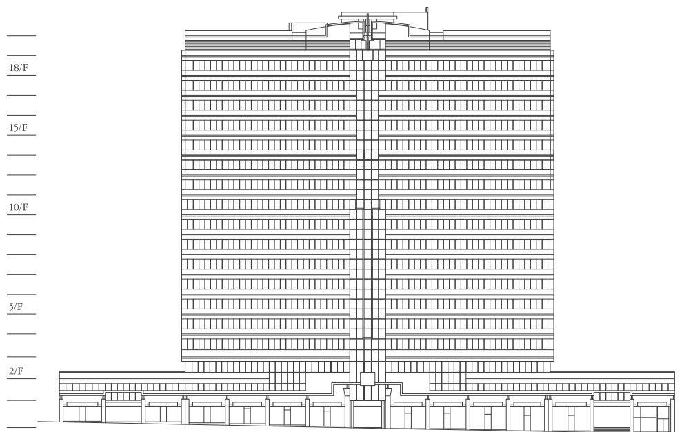
Hankow Road Elevation
